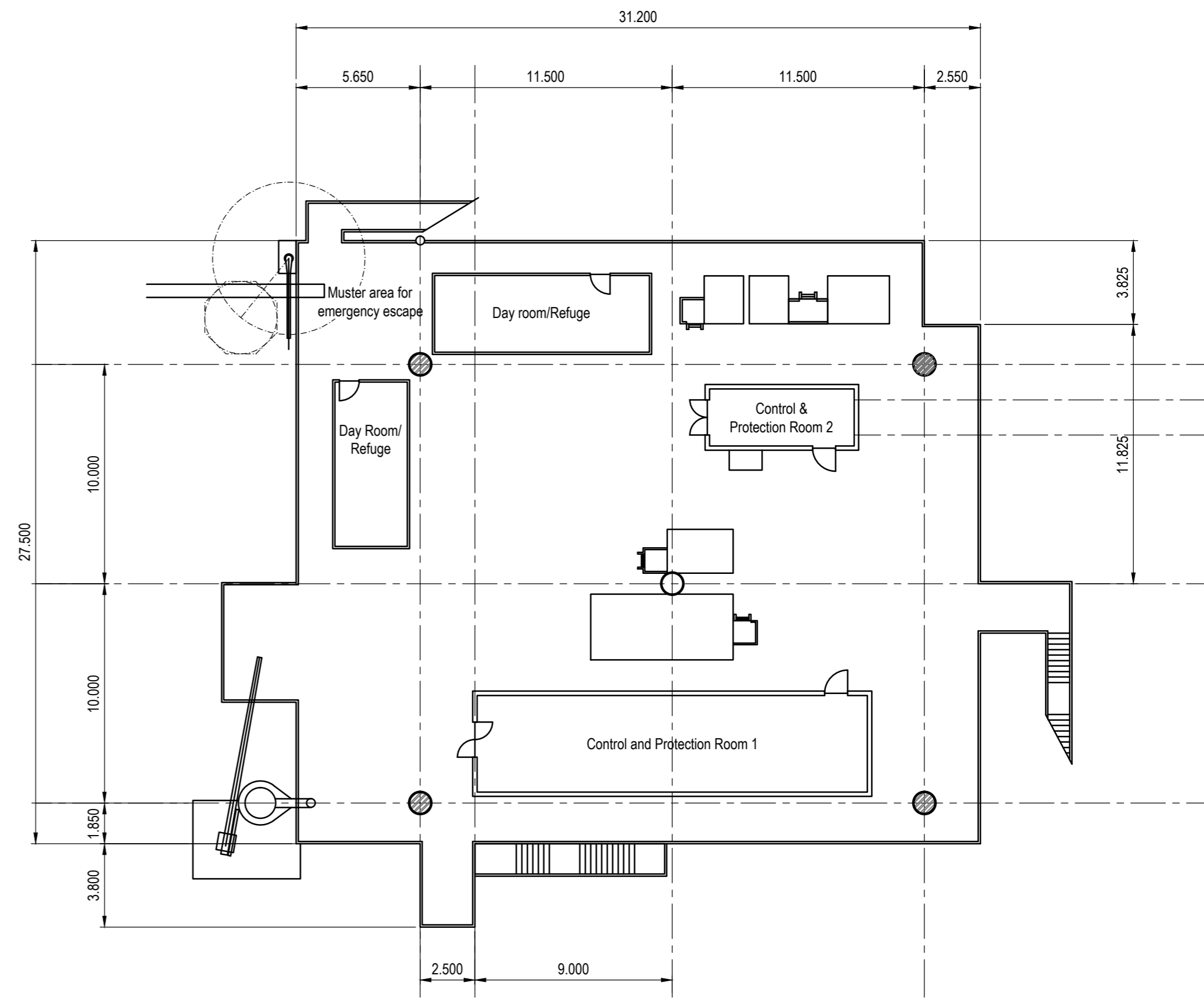
CELLAR DECK
